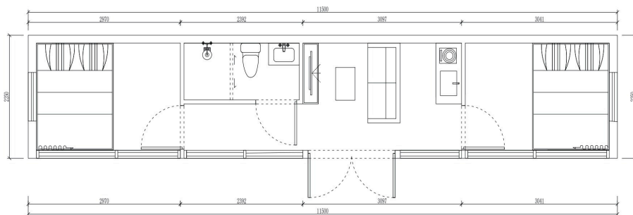
Size: 11500*2250*2450mm Area of structure: 25.8m 2 Accommodate up to : 4-6 people
