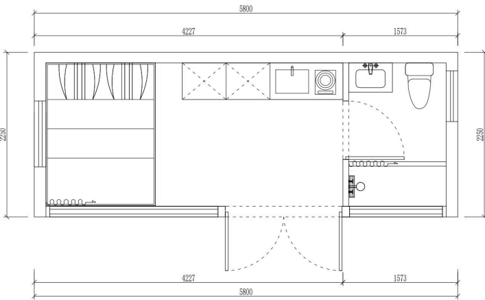
Size: 5800*2250*2450mm Area of structure: 13m 2 Accommodate up to : 1-2 people
