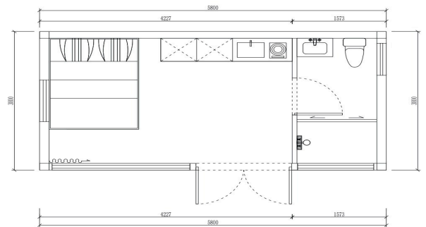
Size: 5800*3000*3200mm Area of structure: 17.4m 2 Accommodate up to: 1-2 people
